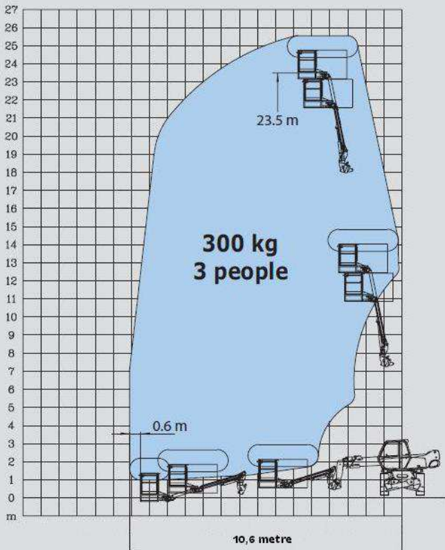
Rotation on rail track fully extended with aerial jib platform
