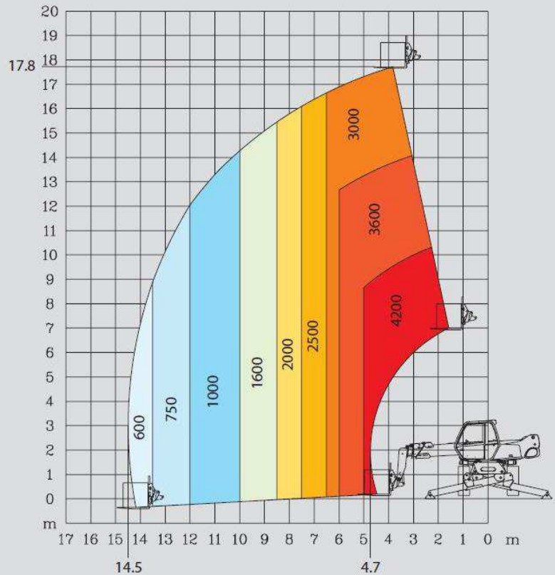
Rotation on stabilisers fully extended with forks
